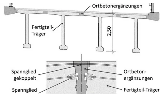
A cross-section and longitudinal section of the three large bridges at Boli, Mettlen and Linden. Source: INGE A4SZ
