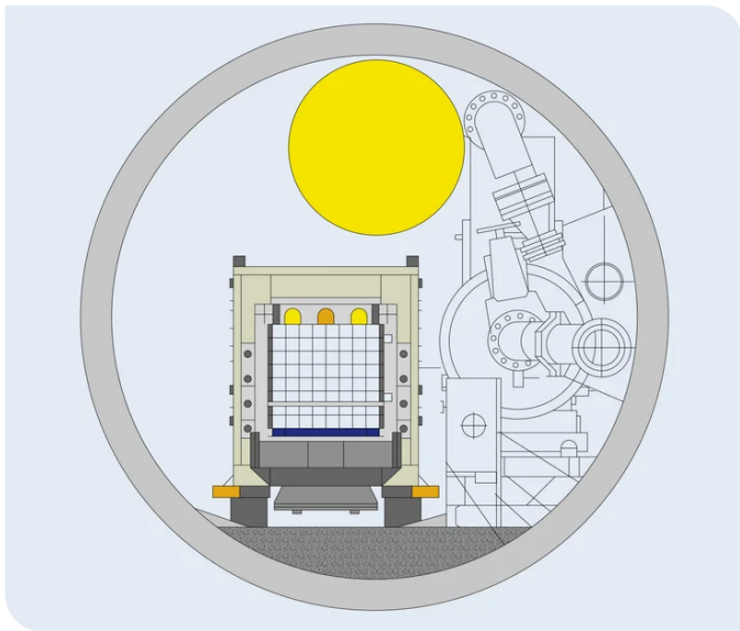
The space conditions in the tunnel cross-section. Picture: HPTJV
