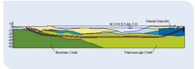
Geological longitudinal section of the route, from the launch shaft in Goxhill to the reception shaft in Paull. Image: National Grid
